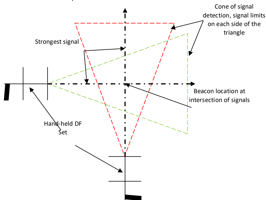
Figure 4-17 Hand-held DF Set usage
