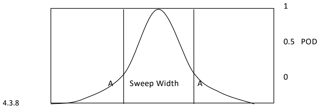
Figure 4-2 Bell curve for POD
