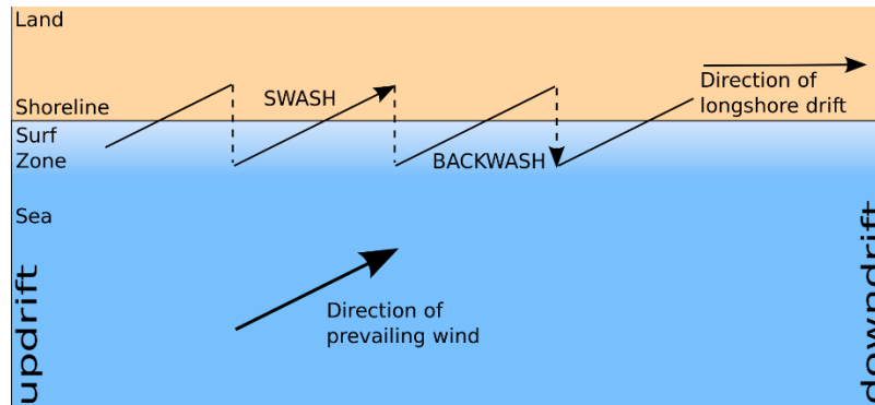
Figure 3-8 Longshore Currents
