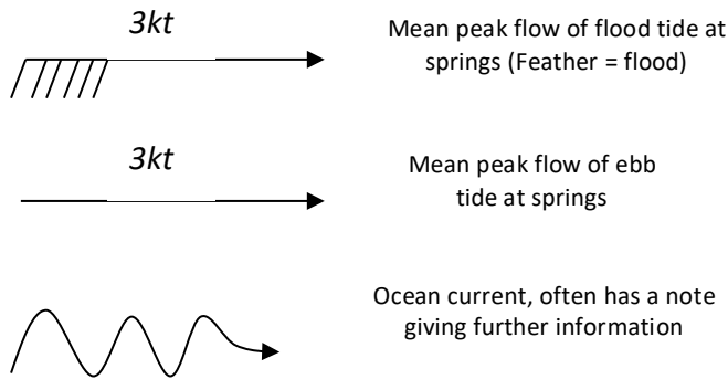
Figure 3-6 Tidal Flow
