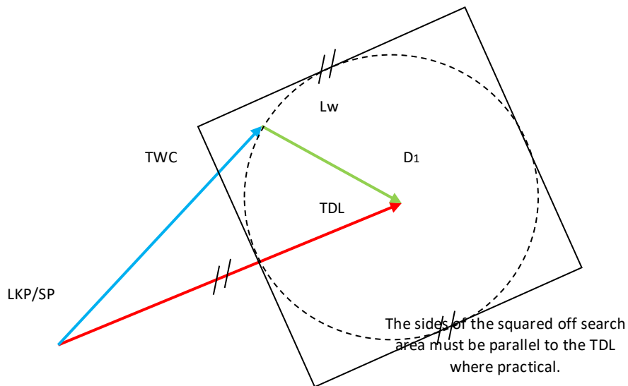
Figure 3-24 Re-computing Datum
