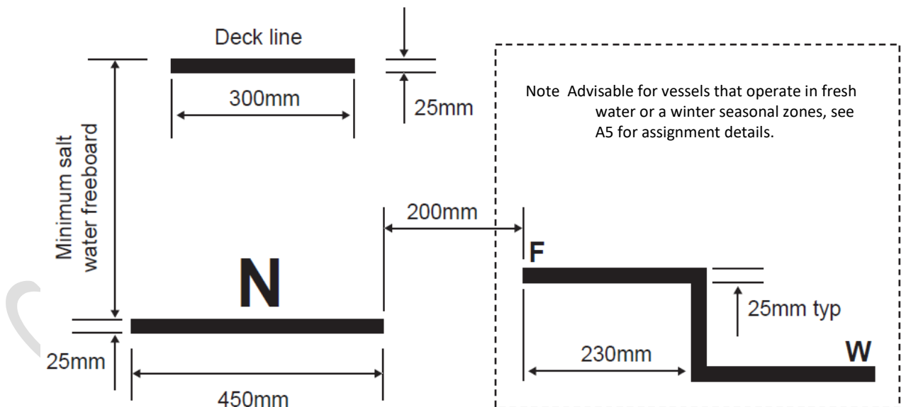
Figure 9 Freeboard mark for vessels ≥24 m in length
