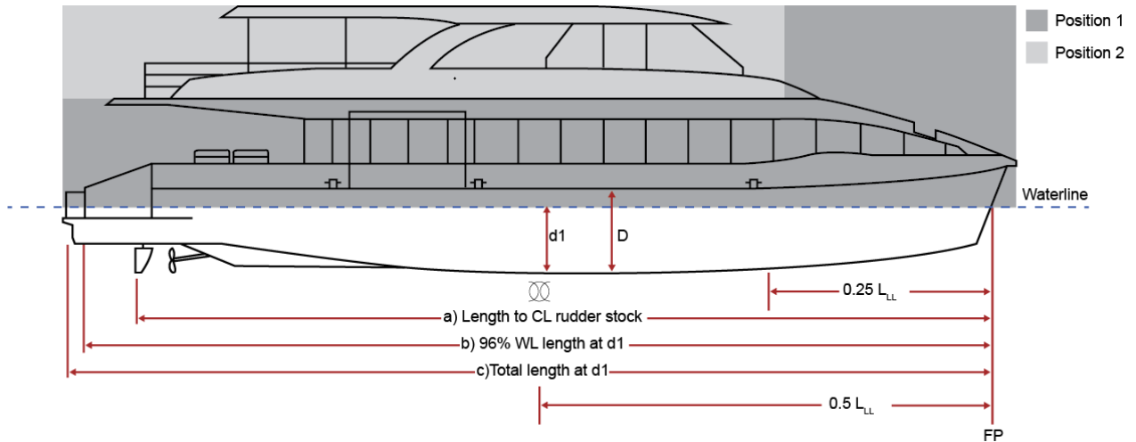
Figure 2 Position 1, Position 2, and standard height of superstructure diagram for a typical vessel \geq 24 m with two levels of superstructure
