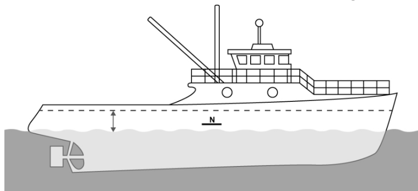
Figure 5 Freeboard mark position, with a compliant loading condition
