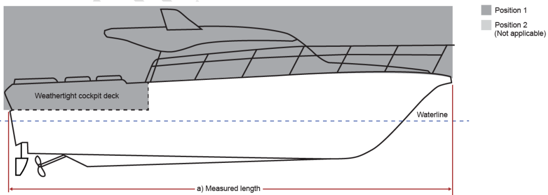
Figure 1 Position 1, and standard height of superstructure diagram for a typical <12 m vessel
