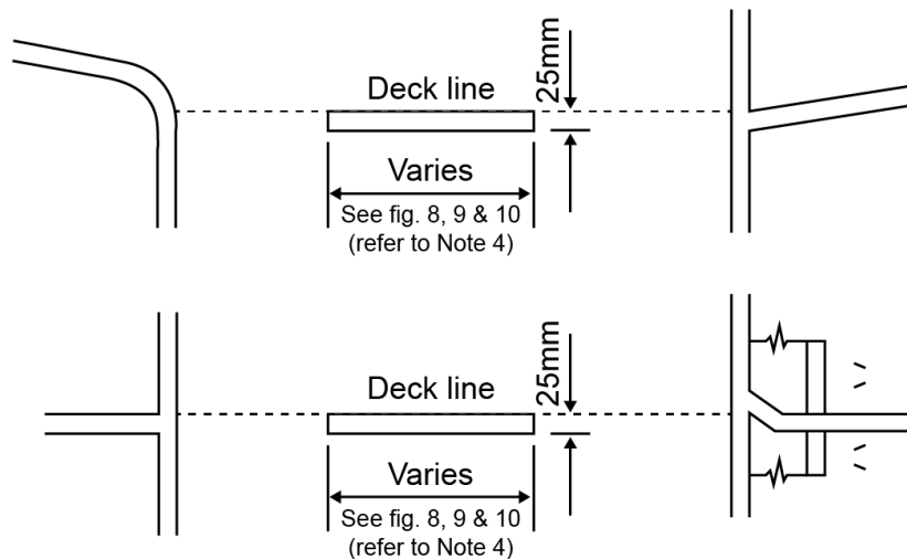
Figure 7 Deck line for all vessels
