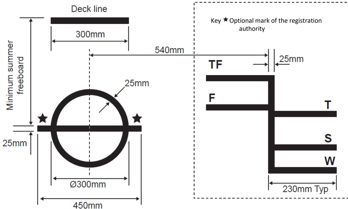
Figure 10 - Deck line and Load Line Mark
