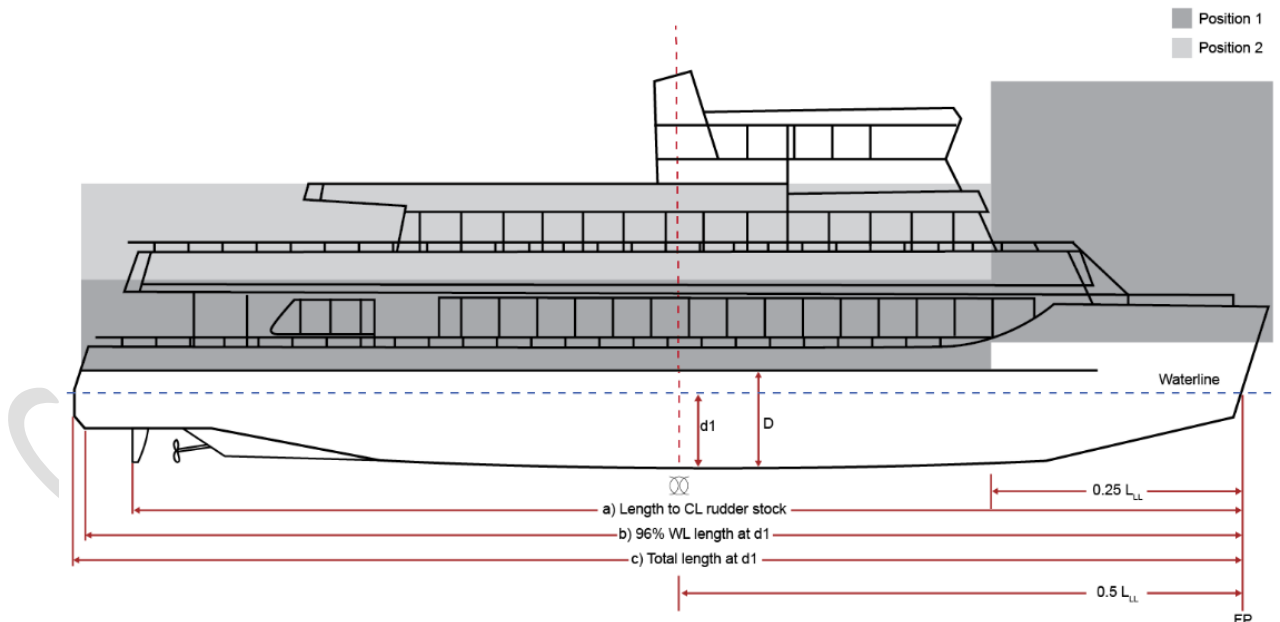
Figure 3 Position 1, Position 2, and standard height of superstructure diagram for a typical vessel \geq 24 m with three levels of superstructure (load line length vessel)
