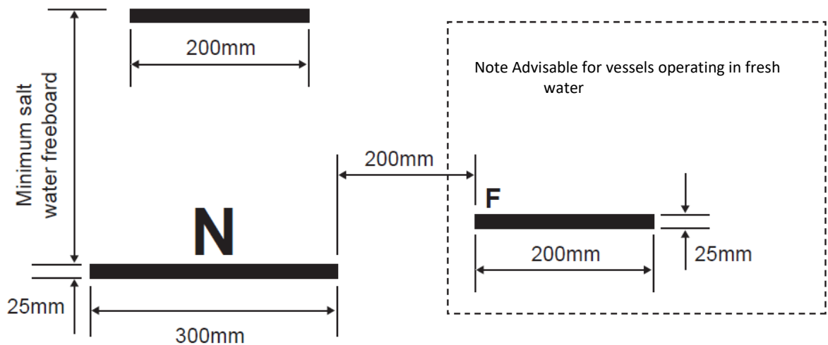
Figure 8 Freeboard mark for vessels <24 m in length
