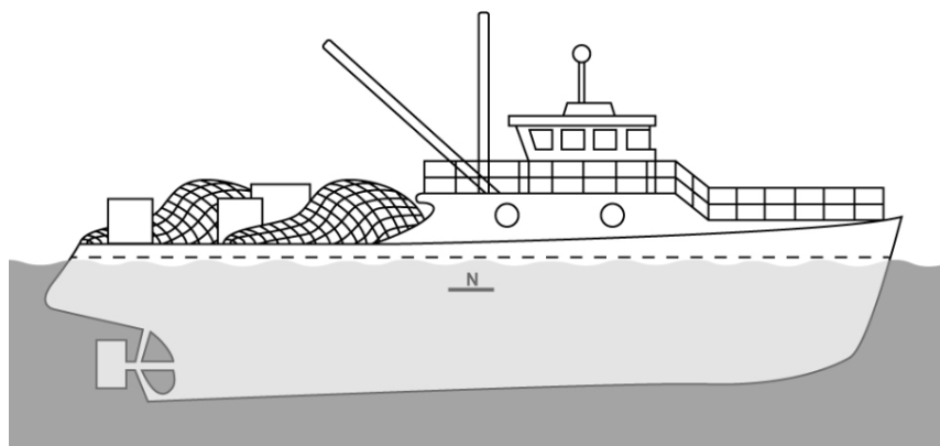
Figure 6 Non-compliant loading condition with the freeboard mark submerged
