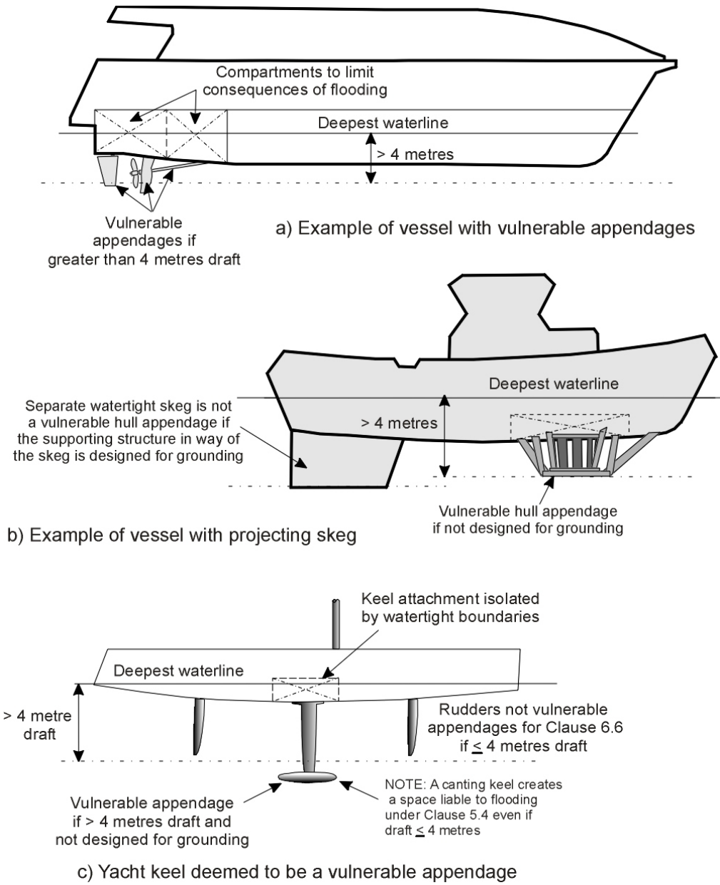
Figure 5 — Vulnerable appendages
