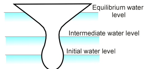
c) Reduced intermediate waterplane area
