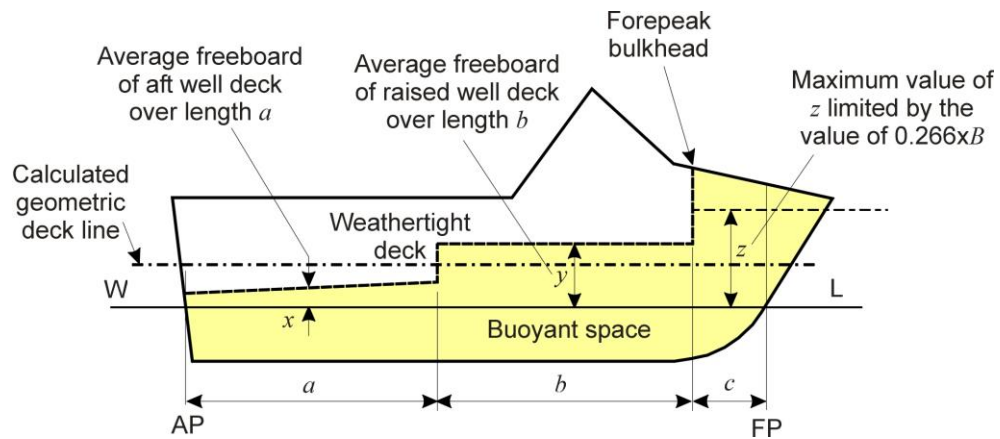
Figure L.1—Geometric freeboard
