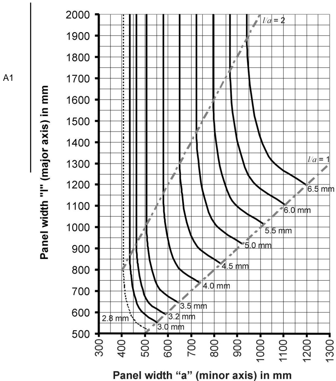
Figure 10 — Minimum thickness of fuel tanks plated in carbon steel for heads not exceeding 2.5 m
