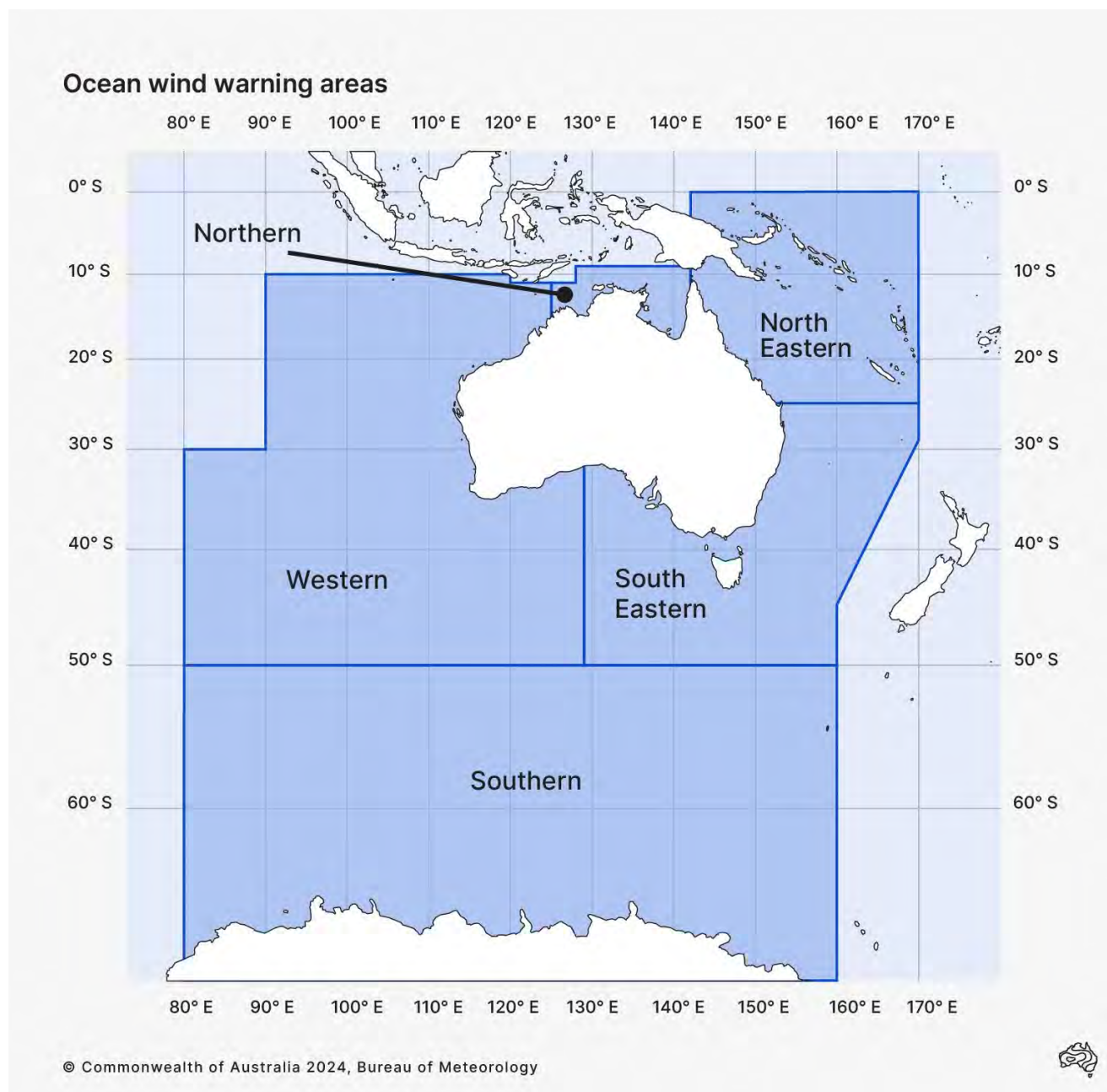
Figure 7 - Ocean wind warning areas
