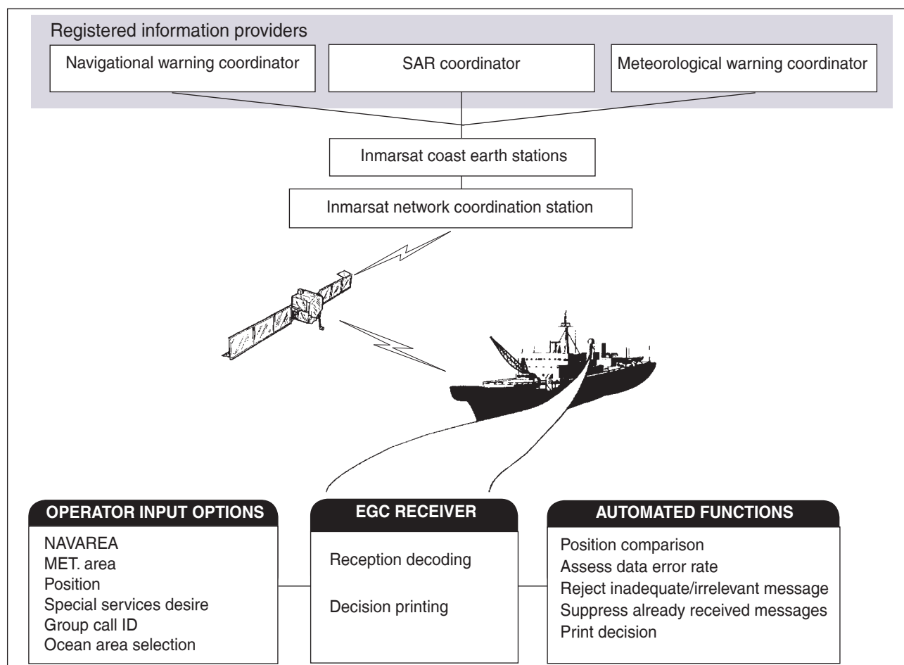
Figure 15 - International SafetyNET Service System Concept
