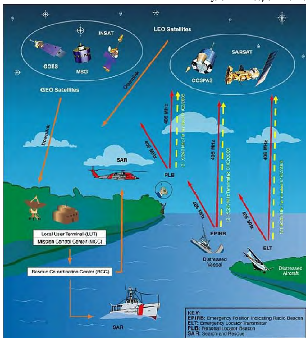
Figure 18 — Basic concept of the Cospas–Sarsat system
