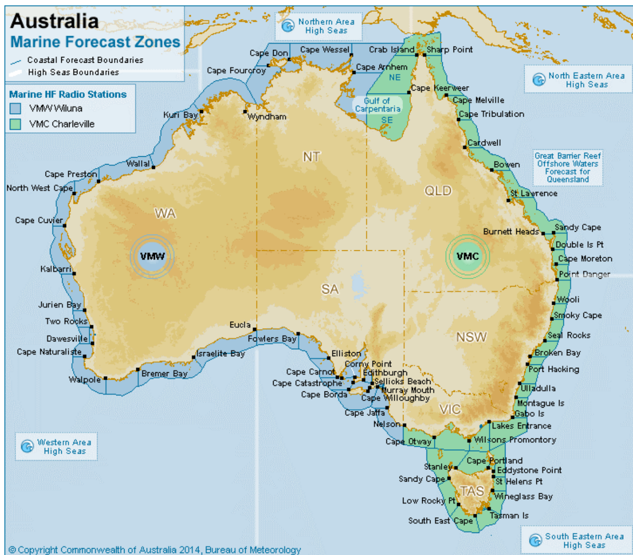
Figure 36 — Forecast areas for high seas
