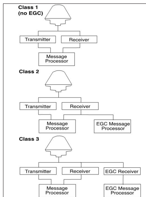
Figure 14 — Classes of mobile earth stations
