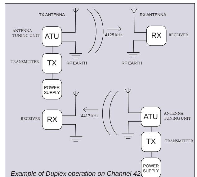
Figure 4 — Duplex operation
