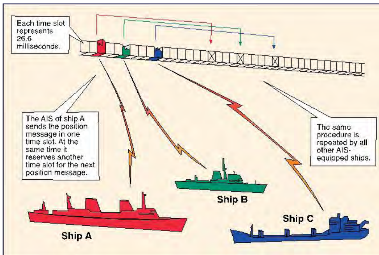
Figure 22 — Principles of SOTDMA
