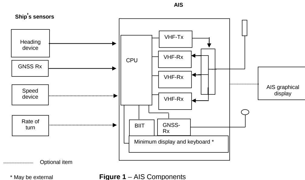
Figure 1 – AIS Components
