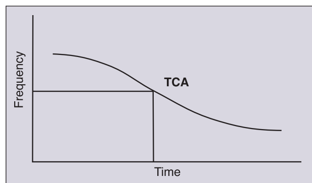
Figure 16 — Doppler Curve
