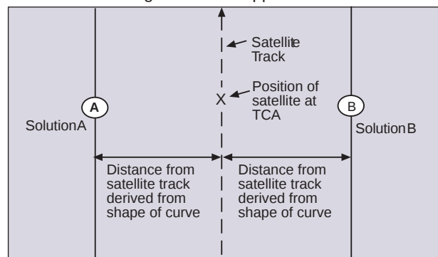
Figure 17 — Doppler Mirror Positions
