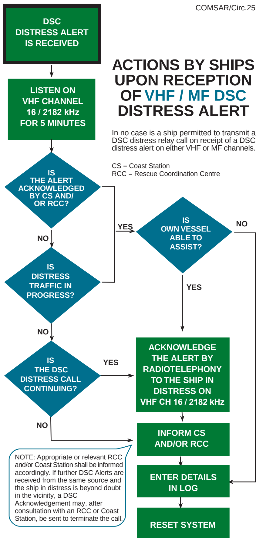
Figure 31 — Action on receipt of a MF or VHF DSC distress alert
