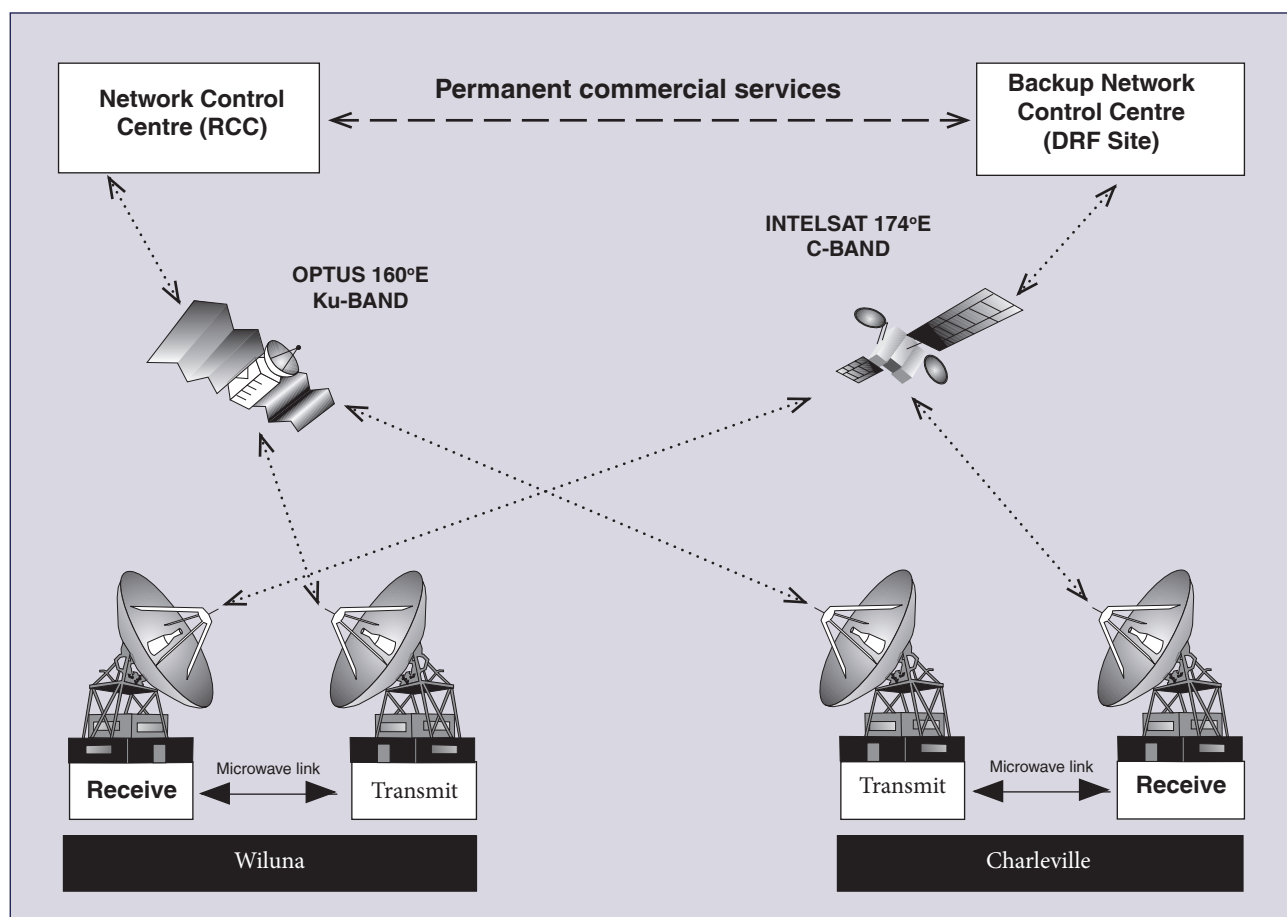
Figure 8 — AMSA HF DSC Network
