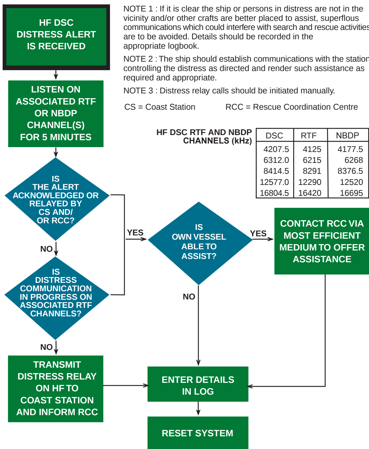
Figure 32 — Action on receipt of an HF DSC distress alert
