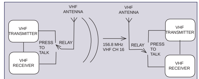
Figure 3 — Simplex operation
