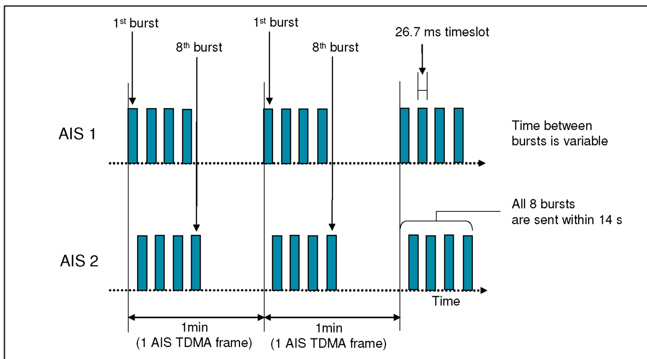
Figure 27 — AIS-SART transmit burst sequence in Active Mode
