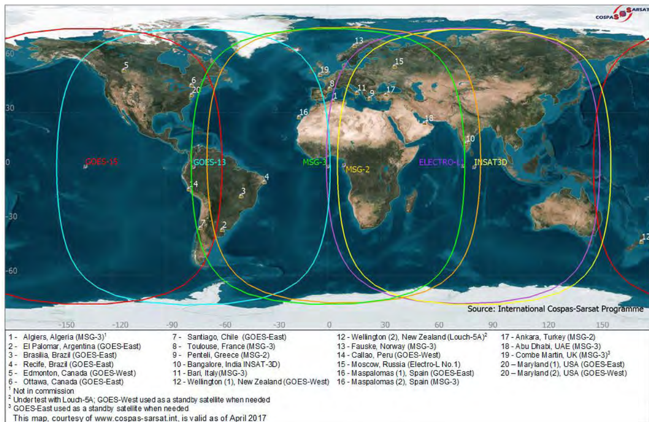
Figure 21 — 406 MHz GEOSAR Satellite Coverage and GEOLUTs
