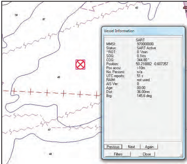
Figure 26 — AIS-SART indication on chart display
