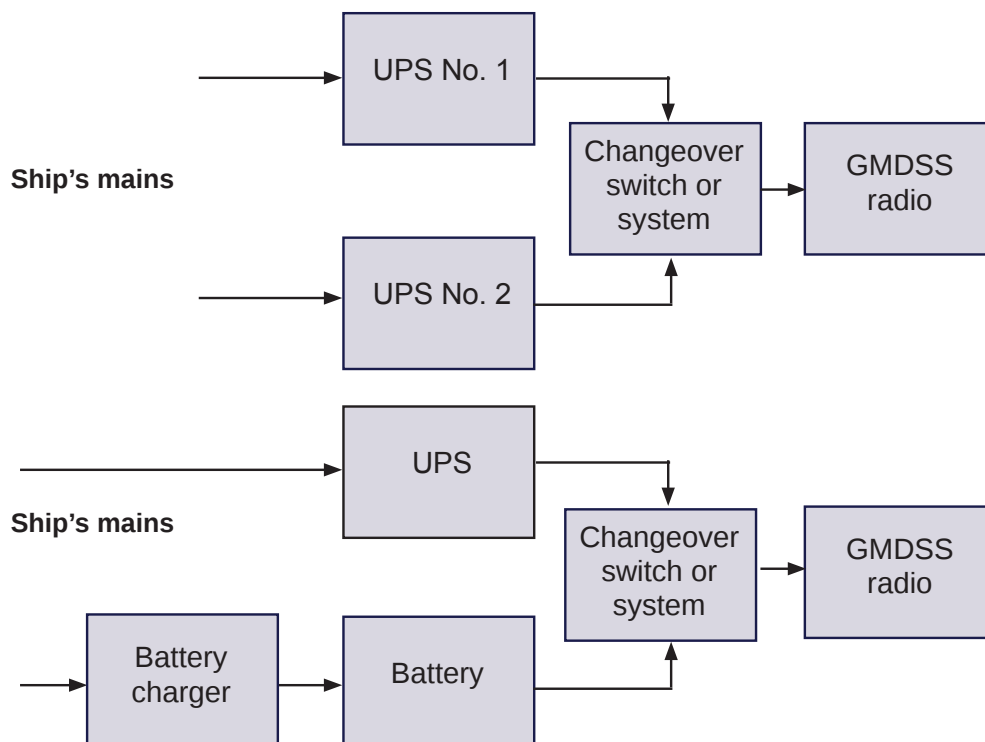
Figure 33 — Typical Uninterruptible Power Supplies
