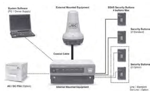
Figure 12 — Typical Inmarsat-C system
