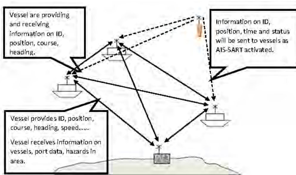
Figure 1 – AIS system overview
