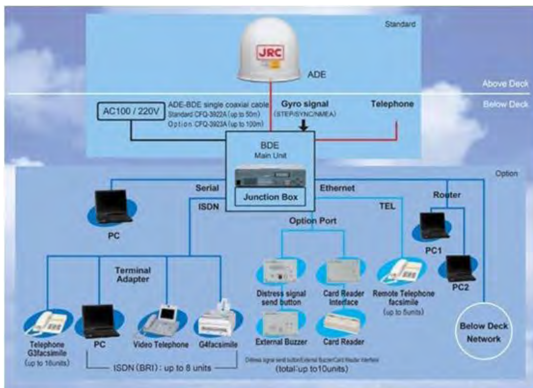
Figure 11 — Typical Inmarsat Fleet 77 installation
