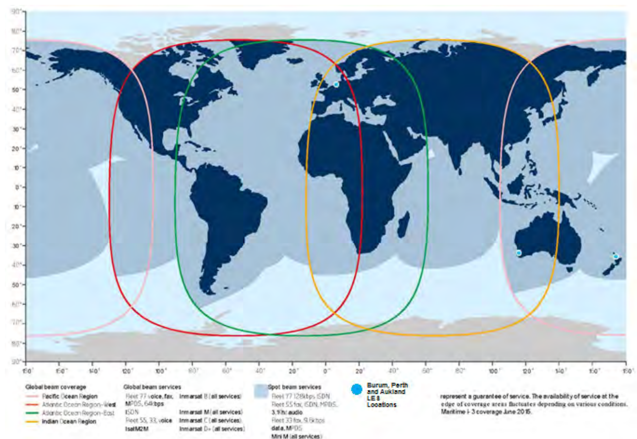
Figure 10 — Inmarsat global coverage applicable to GMDSS (Image courtesy of www.inmarsat.com )
