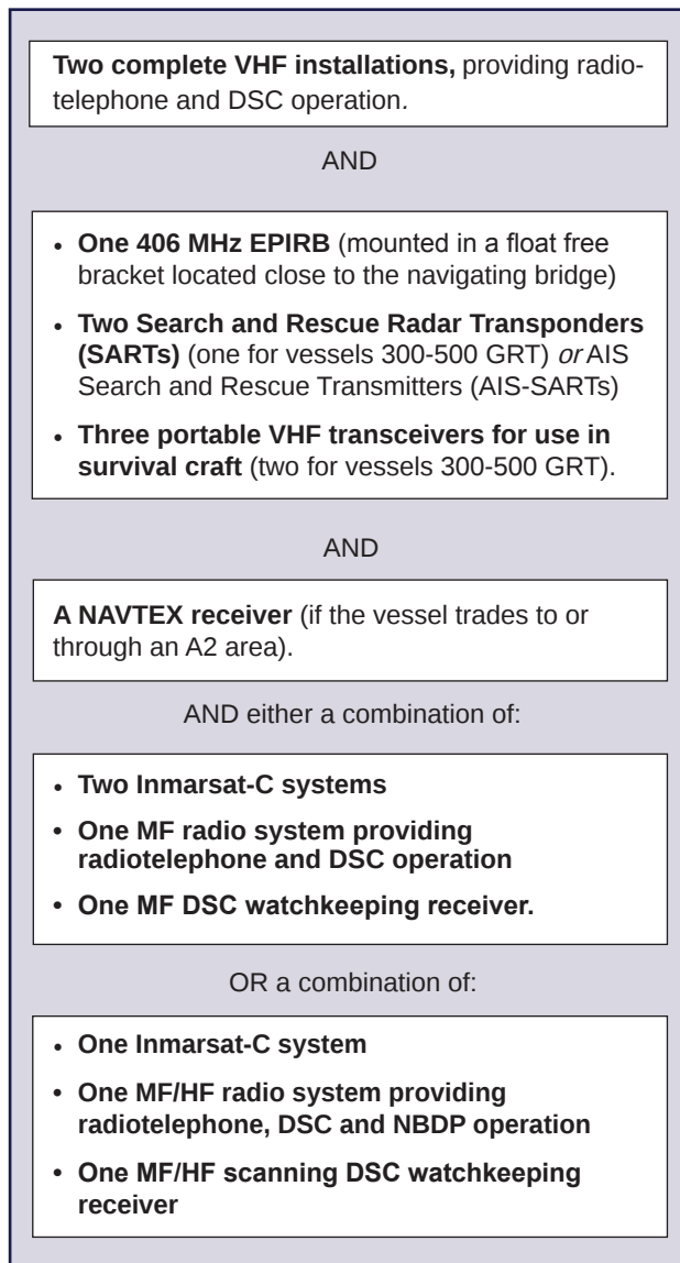
Figure 9 — Equipment required for Australian GMDSS vessels (without an onboard maintainer)
