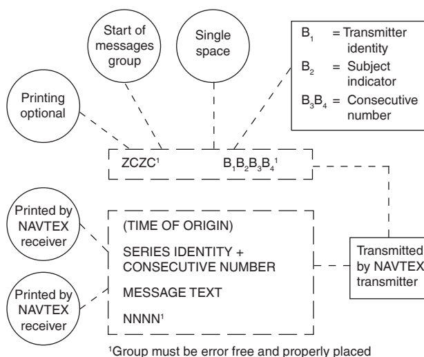
Figure 29 — Format of NAVTEX Message
